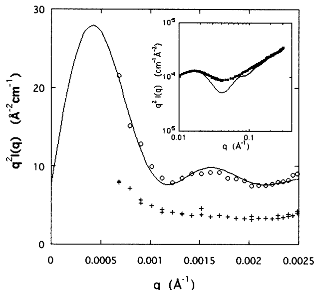
FIG. 4. Kratky representation of the light scattering data for an aggrecan-HA complex. Lower data set is from freshly prepared aggrecan-HA mixture. The inset shows similar representation for aggrecan bottlebrush in the SAXS region.
