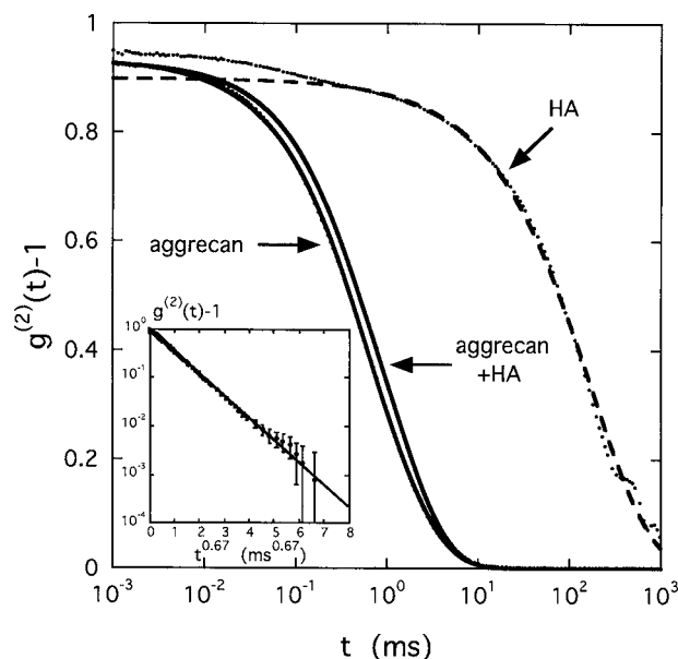
FIG. 5. DLS correlation functions at 90° scattering angle for solutions of aggrecan and aggrecan with HA, as well as of pure HA at 1% ( T=25 °C). Aggrecan concentration of 0.2%, aggrecan/HA ratio of 100. The inset shows fit to g^{(2)}(t)-1 vs t^{2/3} for the aggrecan solution.
