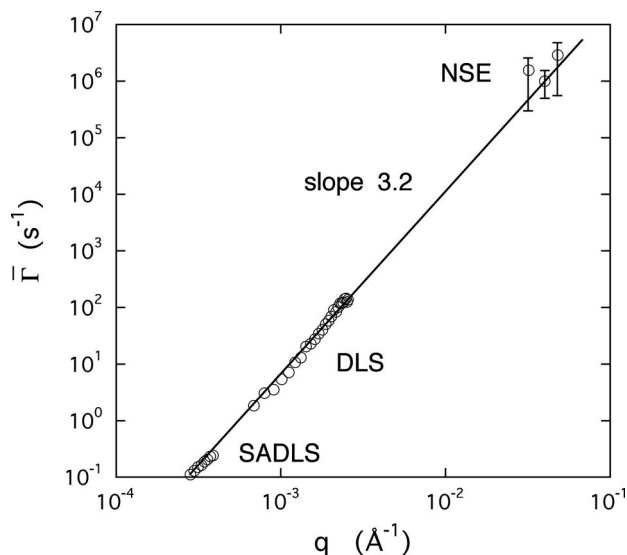
FIG. 7. Relaxation rate \bar{\Gamma}(q) of a 0.6% aggrecan solution measured by SADLS, DLS, and NSE. The slope of the power law fit through the data points is 3.2.
