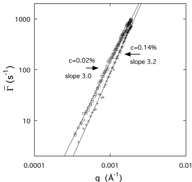
FIG. 6. Relaxation rate \bar{\Gamma}(q) for aggrecan solutions at 0.0002 and 0.0014 g/cm 3 , measured by DLS.
