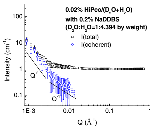
Fig. 3. SANS scattering profiles from a suspension for which the contrast between surfactant and solvent has been matched by mixing D 2 O with H 2 O in the ratio 1:4.394 by weight. The concentration of HiPco is 0.02 wt% and the ratio of nanotube-to-surfactant is 1:10. After subtracting the incoherent background, the -2 slope at low Q is quite apparent and a fairly convincing -1 slope above Q = 0.003 \text{\AA}^{-1} is observed.
