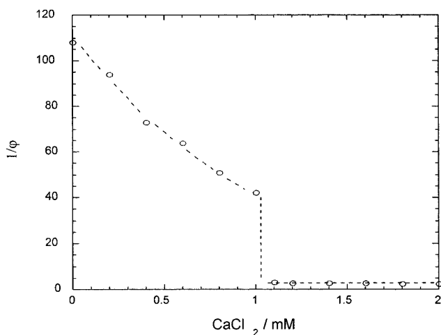
Fig. 1. Dependence of the equilibrium swelling degree of a sodium polyacrylate hydrogel on the \text{CaCl}_2 concentration in 40 mM NaCl solution.
