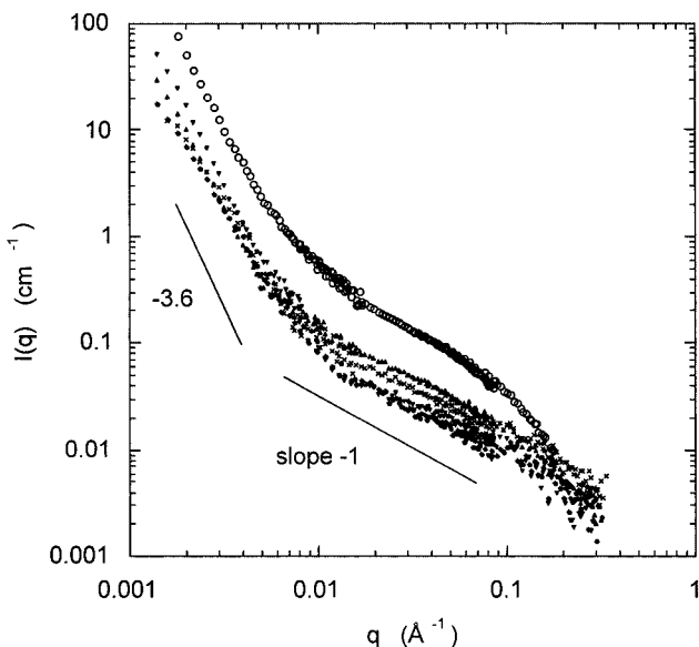
Fig. 5. Plot of SANS spectra for sodium polyacrylate gels swollen in 40 mM NaCl solution with various calcium contents indicated in box. The straight lines indicate slopes of -3.6 and -1 , respectively. \text{CaCl}_2 concentration in equilibrium bath: \bullet : 0.75 mM; \circ : 0.85 mM; \times : 1.0 mM; + : 1.2 mM; \Delta : 1.7 mM; \nabla : 2.0 mM.
