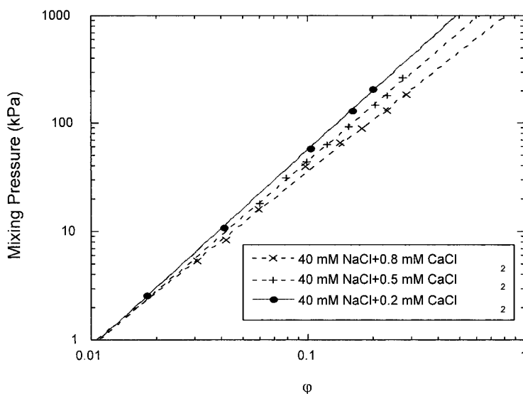
Fig. 3. Osmotic mixing pressure of polyacrylate hydrogels as a function of polymer volume fraction \phi , in solutions containing 40 \text{ mM NaCl} and different amounts of \text{CaCl}_2 . The slopes of the straight lines through the experimental data points are 1.81 ( 0.2 \text{ mM Ca} : \bullet ), 1.71 ( 0.5 \text{ mM Ca} : + ) and 1.59 ( 0.8 \text{ mM Ca} : \times ).
