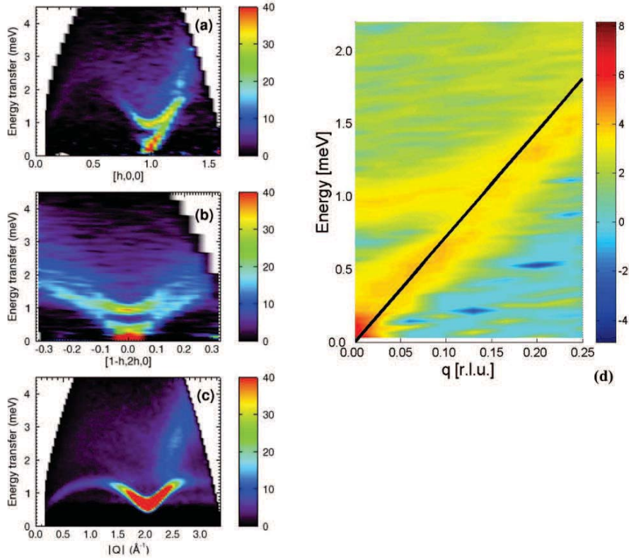
Figure 1. Cuts of scattered intensity contours in energy–wavevector space for hcp ^4\text{He} . (a) For Q along \langle 100 \rangle , (b) for Q through the (100) reciprocal lattice point in the transverse direction in the basal plane, (c) for the superfluid at P = 24 bar and T = 0.22 K. Intensities have been integrated over the perpendicular direction to the cut by 0.01 reciprocal lattice units. (d) Expanded plot of cut shown in (a) to show detail of ‘collision’ and merging of upper longitudinal mode and LA phonon mode.
